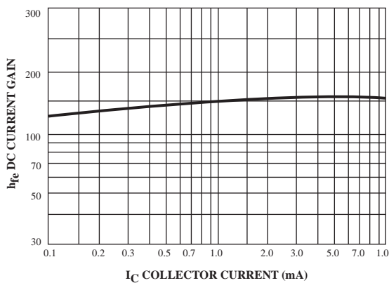
FIG.9 Current Gain
