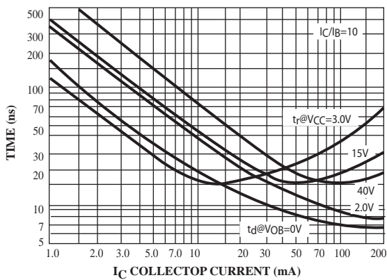
FIG.5 Turn-On Time
