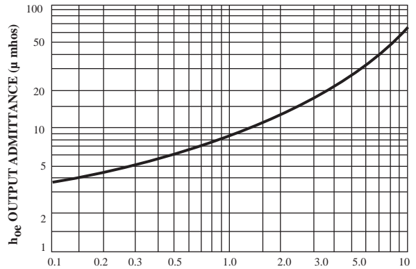
FIG.12 Output Admittance
