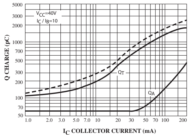
FIG.4 Charge Data
