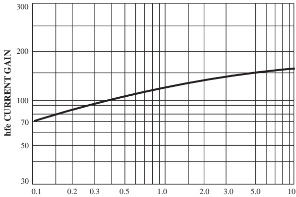
FIG.11 Current Gain
