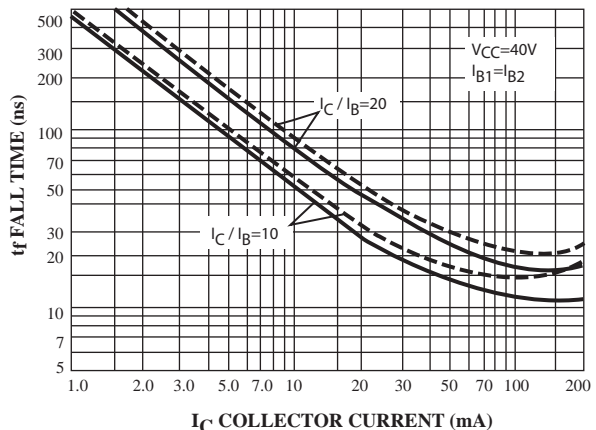
FIG.8 Fall Time
