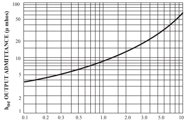
Figure 12. Output Admittance
